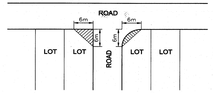
Figure 2: Sight Triangle
