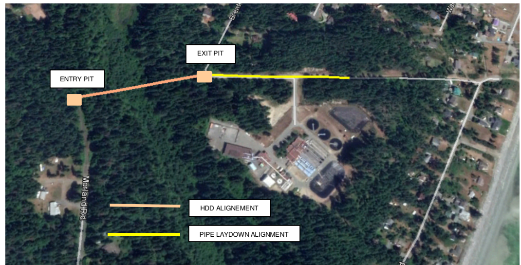
Figure 5 – Lazo Marsh HDD Forcemain Section and Laydown Area
