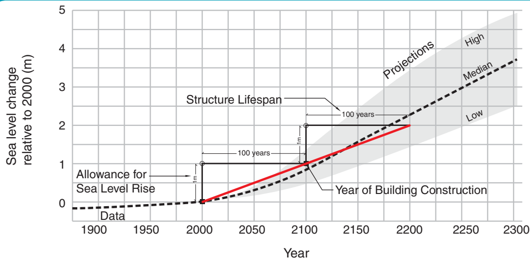
Figure 2 - Sea level rise allowance for structure lifespan (Ausenco Sandwell, 2011)
