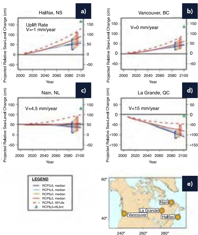
FIGURE 24: Projected relative sea-level change, based on the IPCC Fifth Assessment Report (Church et al., 2013a, b) and utilizing vertical (V) crustal motion (uplift rate, given to nearest 0.5 mm/year) derived from GPS observations indicated in each panel for a) Halifax, b) Vancouver, c) Nain and d) La Grande 1 (James et al., 2014, 2015). Projections are given through the current century for the low-emissions (RCP2.6), intermediate-emissions (RCP4.5) and high-emissions (RCP8.5) scenarios. The projected value at 2100 is also given for the high-emissions plus Antarctic Ice-Sheet reduction scenario (RCP8.5+W.Ant; green triangle). Rectangles show the 90% confidence interval (5 th –95 th percentile) of the average projection over the period 2081–2100 and also include the RCP6.0 scenario; the dashed red line shows the 95 th percentile value for the high-emissions scenario.
