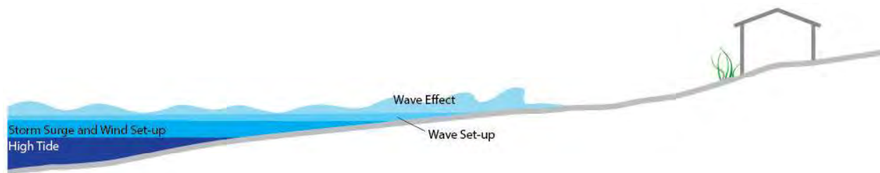
Figure 2-1: Components of total water level (total water level is composed of tide, storm surge, wind set-up, wave set-up and wave runup).
